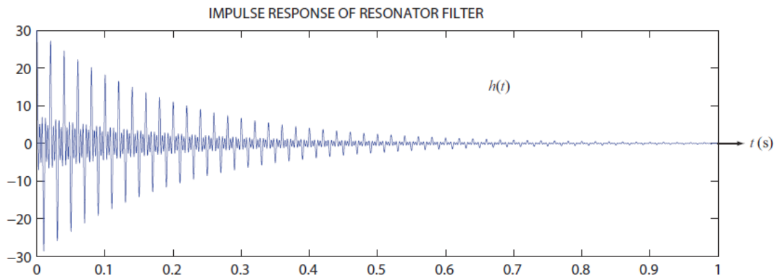
The resonator filter frequency and impulse responses
